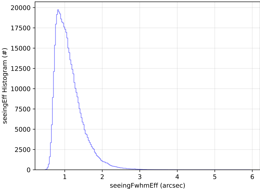
early_u_fpextra2.0_v3.4_10yrs WFD r band: seeingEff Histogram
