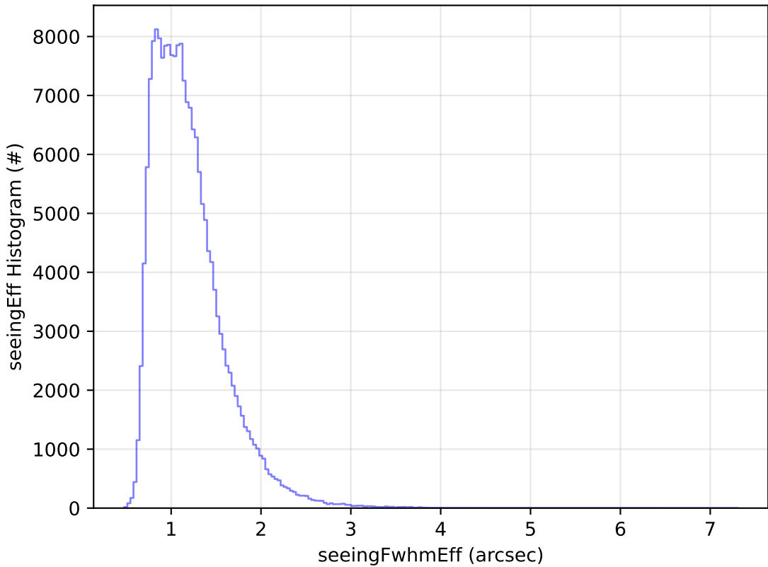
early_u_fpextra2.0_v3.4_10yrs WFD g band: seeingEff Histogram
