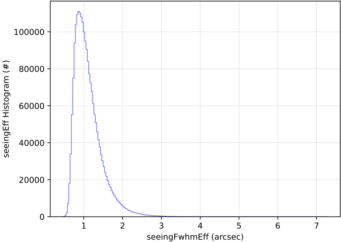
early_u_fpextra2.0_v3.4_10yrs WFD all bands: seeingEff Histogram
