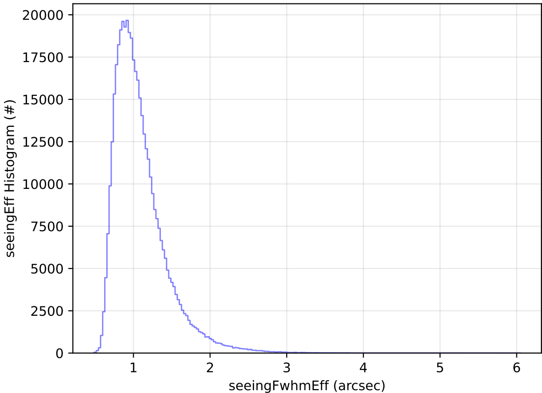
early_u_fpextra2.0_v3.4_10yrs All sky z band: seeingEff Histogram
