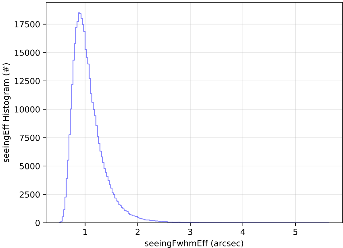
early_u_fpextra2.0_v3.4_10yrs All sky y band: seeingEff Histogram
