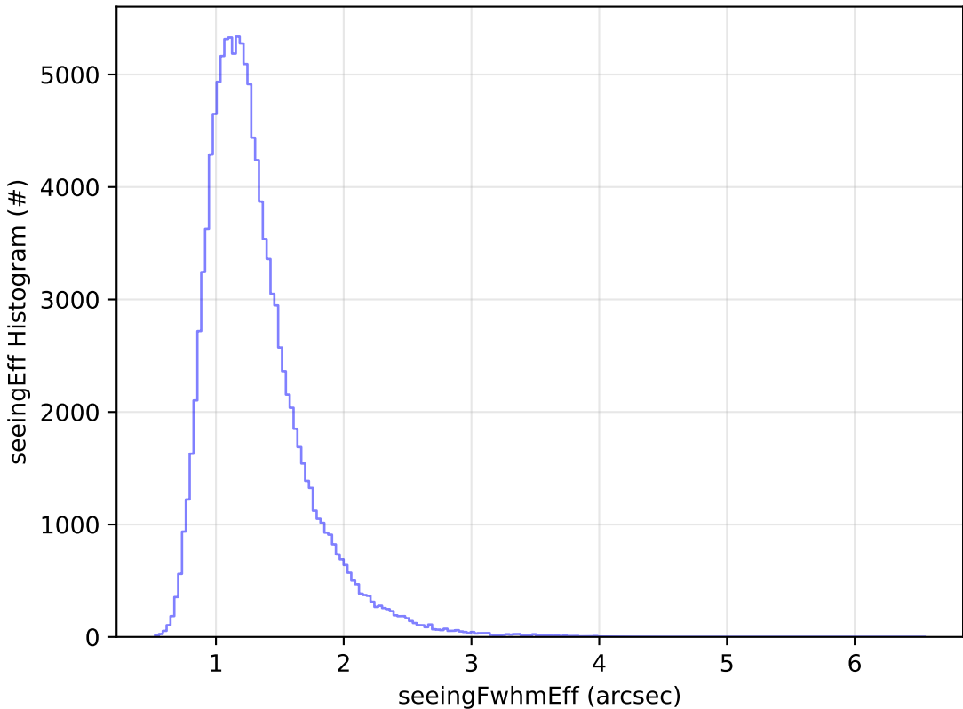
early_u_fpextra2.0_v3.4_10yrs All sky u band: seeingEff Histogram
