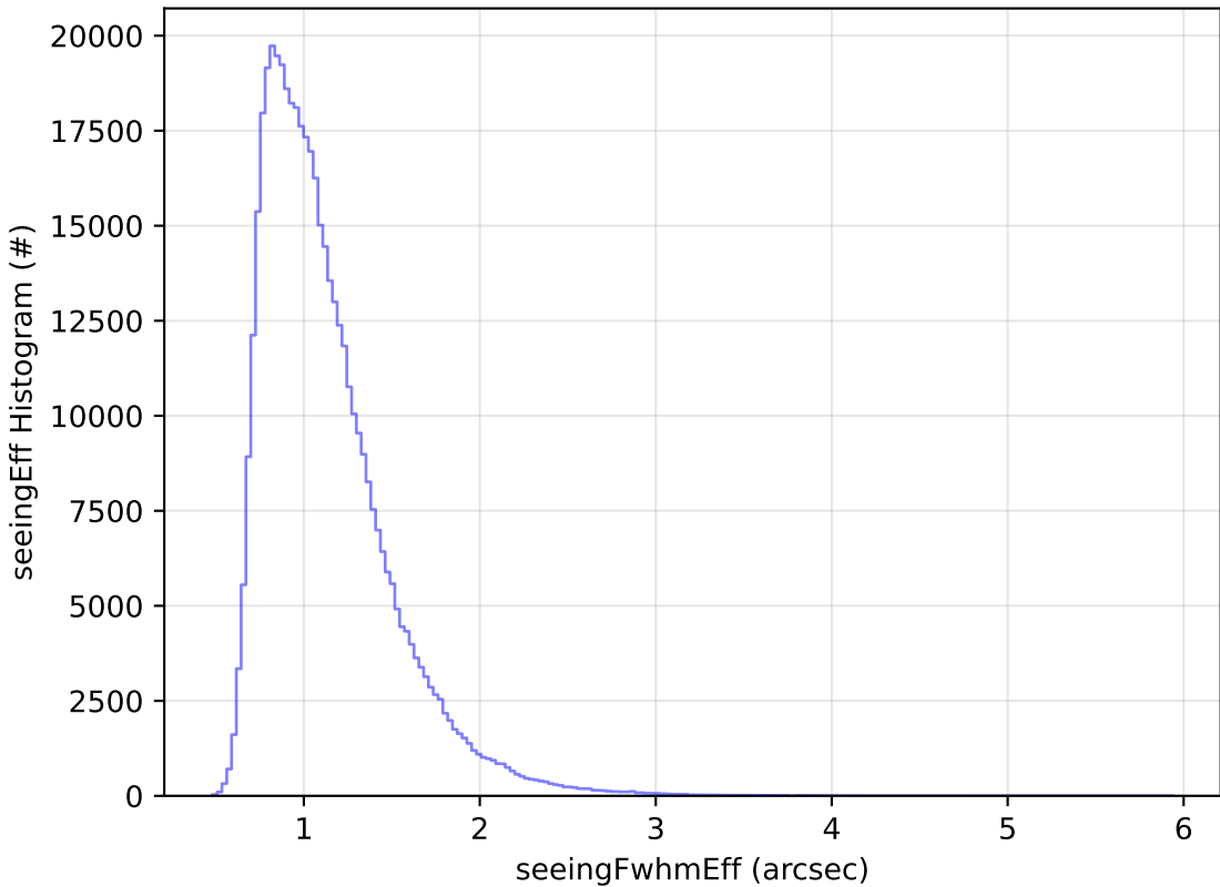
early_u_fpextra2.0_v3.4_10yrs All sky r band: seeingEff Histogram
