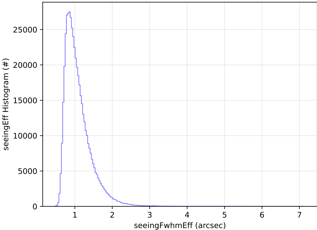
early_u_fpextra2.0_v3.4_10yrs All sky i band: seeingEff Histogram
