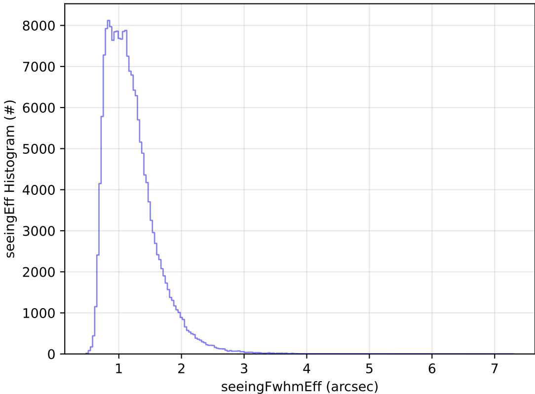
early_u_fpextra2.0_v3.4_10yrs All sky g band: seeingEff Histogram
