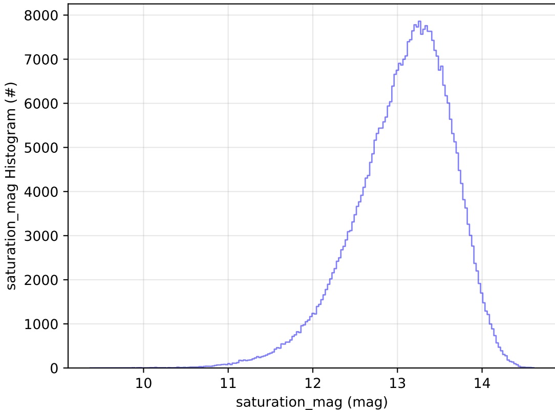
early_u_fpextra2.0_v3.4_10yrs WFD y band: saturation_mag Histogram
