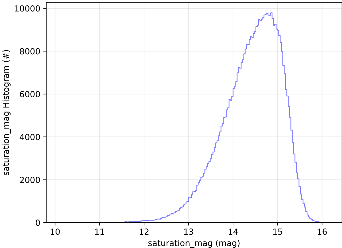
early_u_fpextra2.0_v3.4_10yrs WFD i band: saturation_mag Histogram
