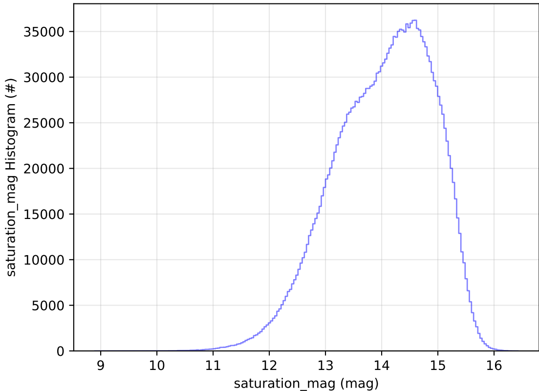
early_u_fpextra2.0_v3.4_10yrs WFD all bands: saturation_mag Histogram
