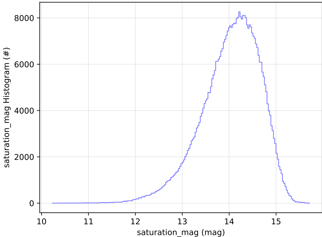
early_u_fpextra2.0_v3.4_10yrs All sky z band: saturation_mag Histogram
