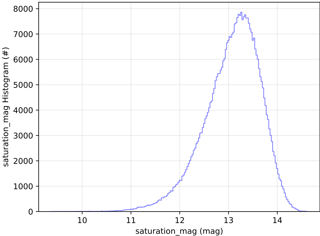
early_u_fpextra2.0_v3.4_10yrs All sky y band: saturation_mag Histogram
