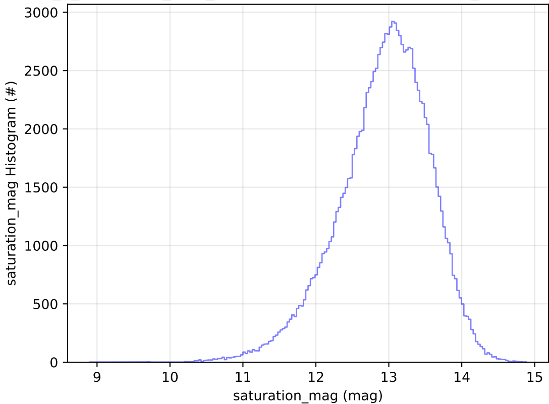
early_u_fpextra2.0_v3.4_10yrs All sky u band: saturation_mag Histogram
