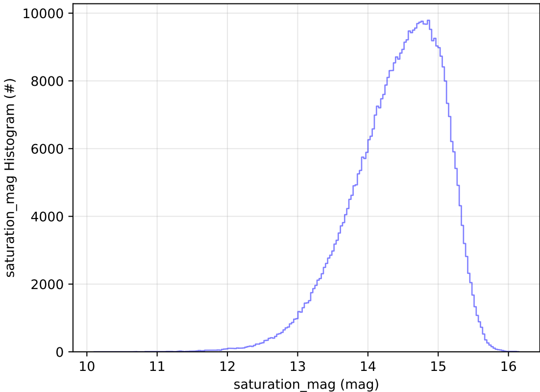
early_u_fpextra2.0_v3.4_10yrs All sky i band: saturation_mag Histogram
