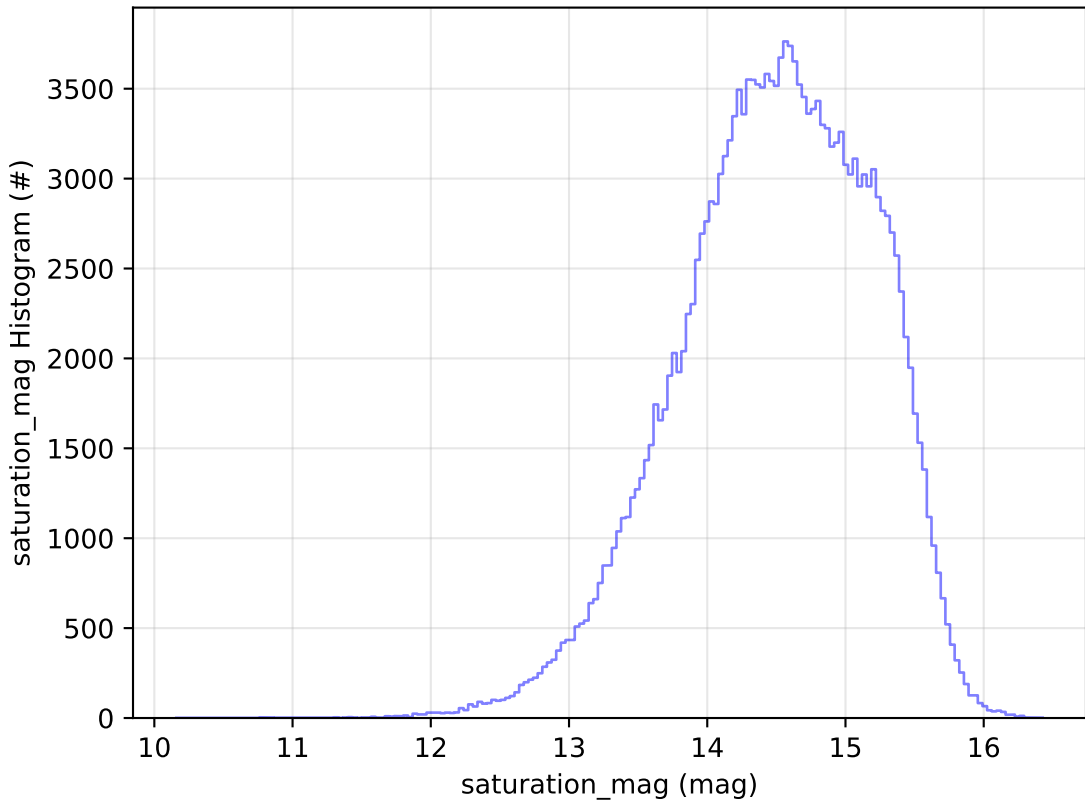
early_u_fpextra2.0_v3.4_10yrs All sky g band: saturation_mag Histogram
