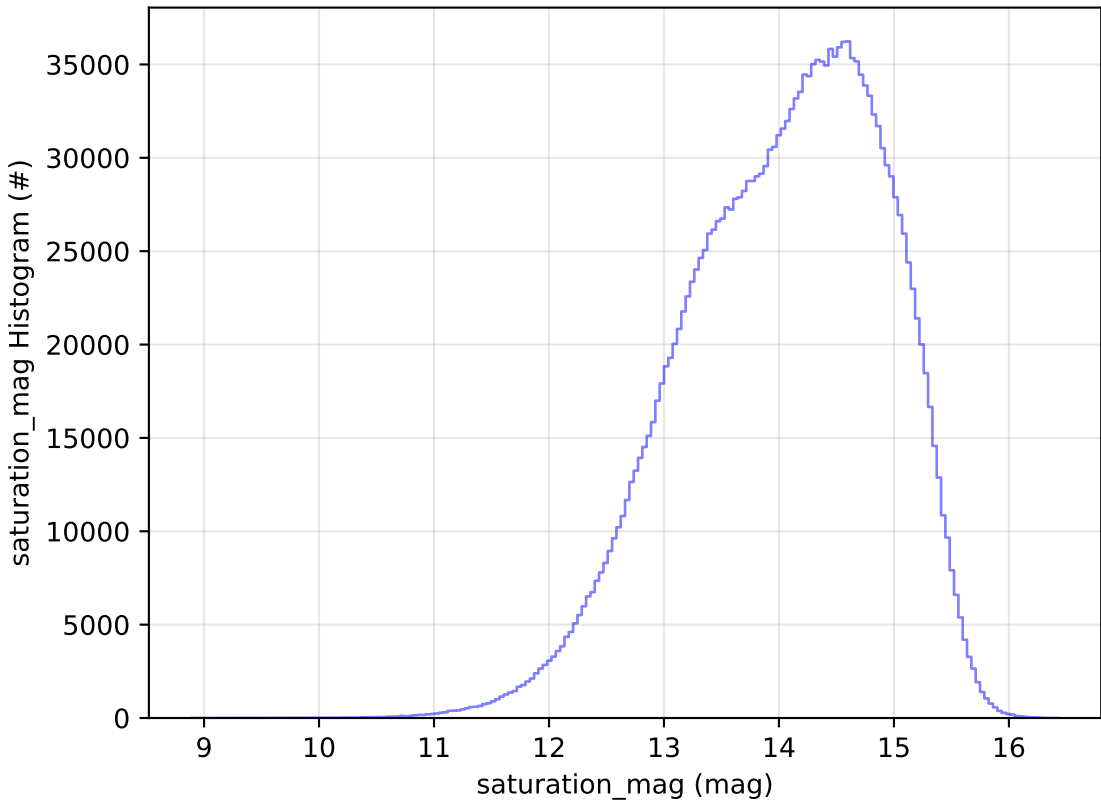
early_u_fpextra2.0_v3.4_10yrs All sky all bands: saturation_mag Histogram
