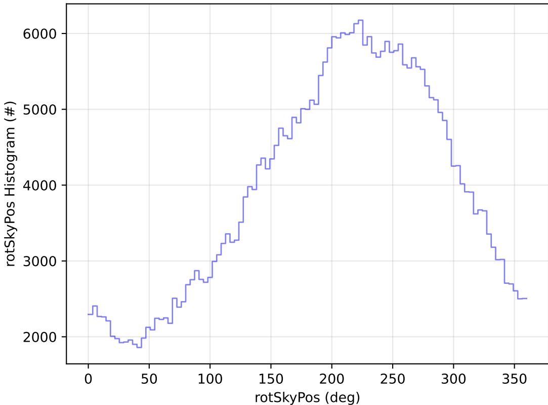
early_u_fpextra2.0_v3.4_10yrs WFD y band: rotSkyPos Histogram
