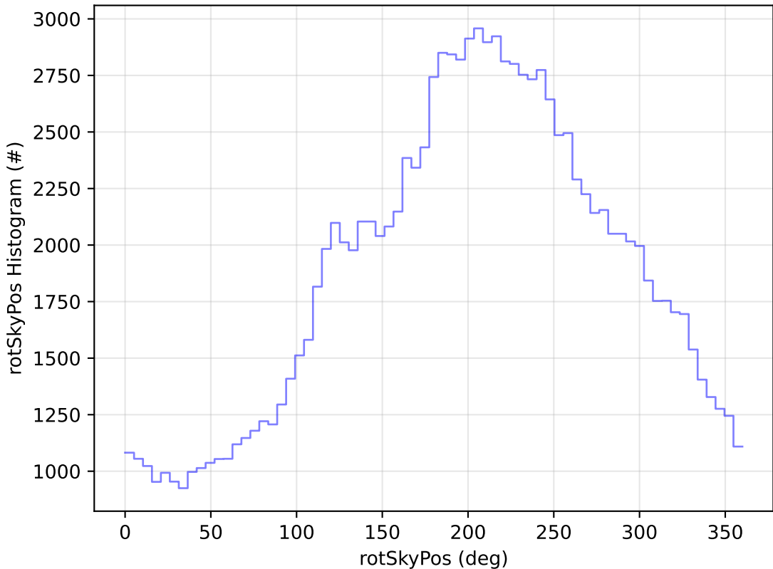
early_u_fpextra2.0_v3.4_10yrs WFD u band: rotSkyPos Histogram
