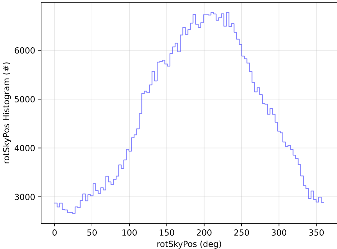
early_u_fpextra2.0_v3.4_10yrs WFD r band: rotSkyPos Histogram
