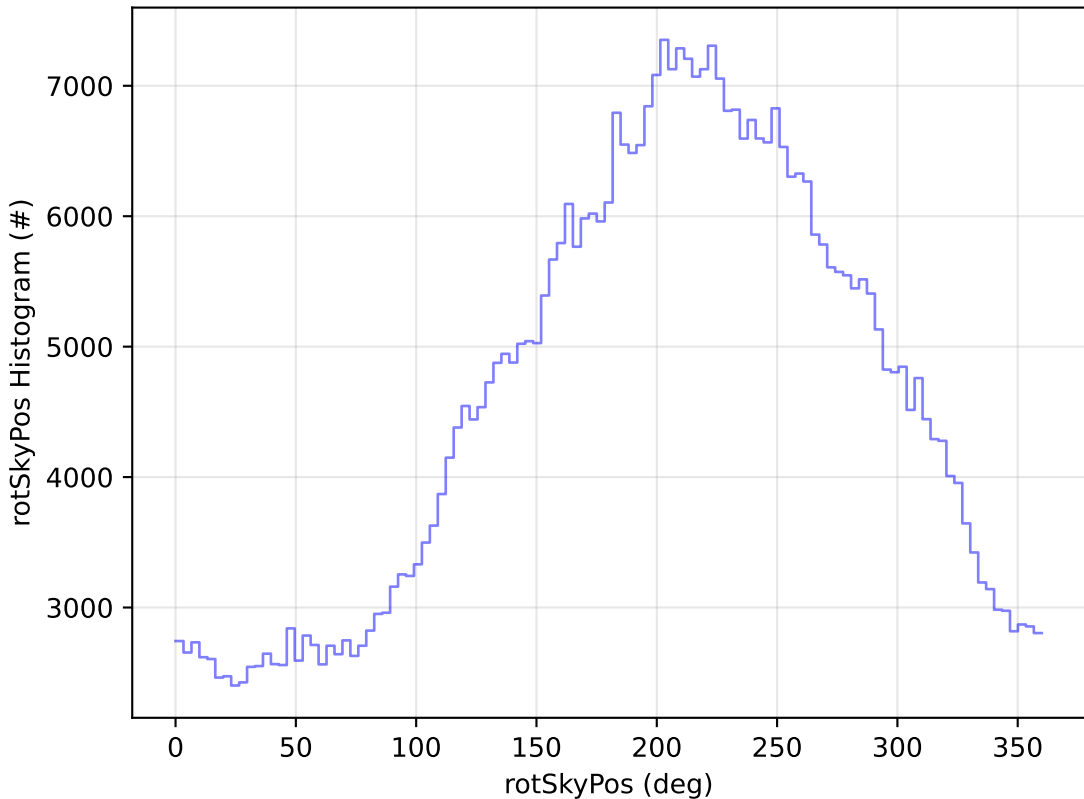
early_u_fpextra2.0_v3.4_10yrs WFD i band: rotSkyPos Histogram
