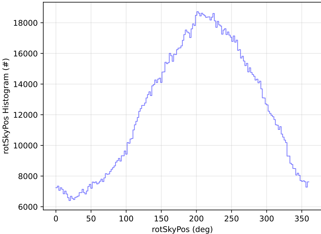
early_u_fpextra2.0_v3.4_10yrs WFD all bands: rotSkyPos Histogram
