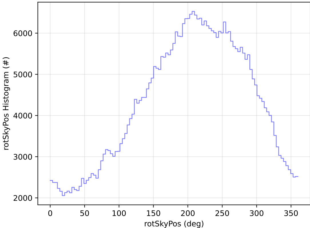
early_u_fpextra2.0_v3.4_10yrs All sky z band: rotSkyPos Histogram
