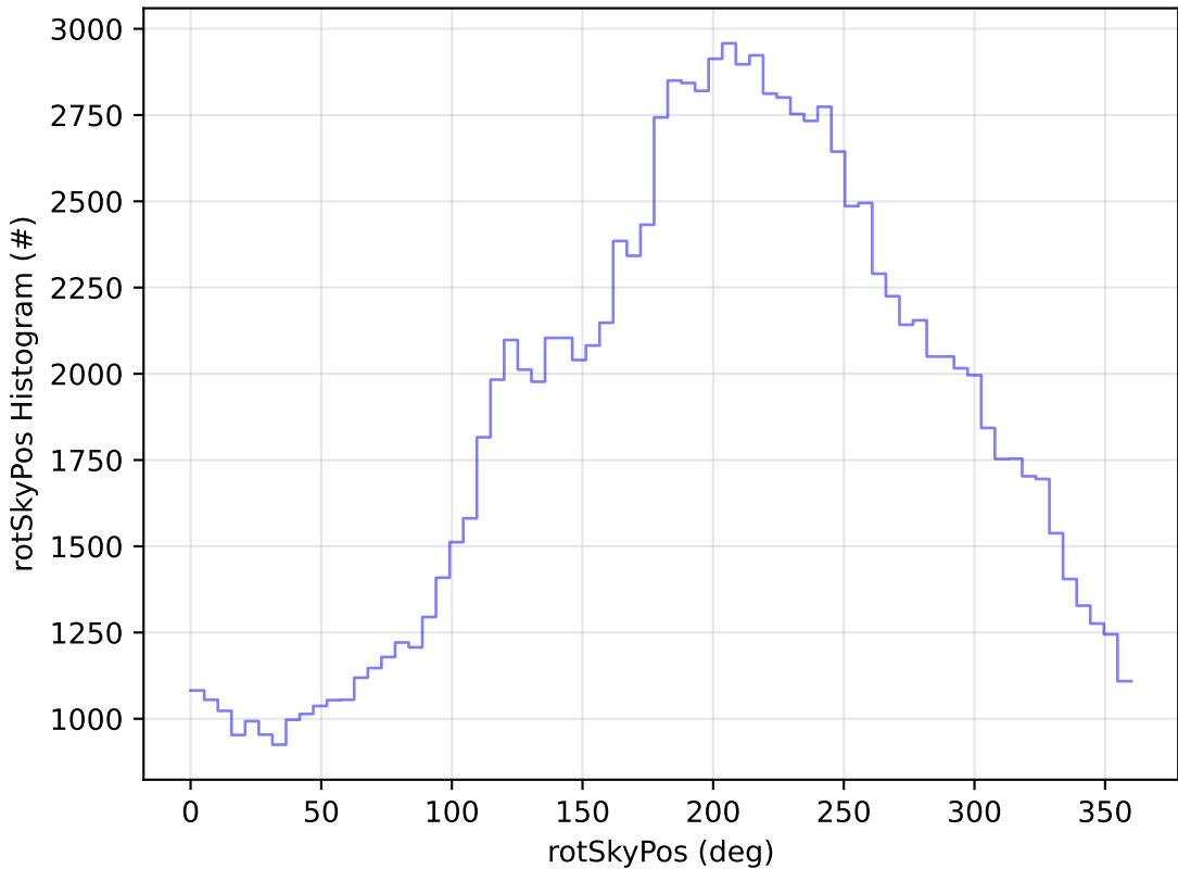
early_u_fpextra2.0_v3.4_10yrs All sky u band: rotSkyPos Histogram
