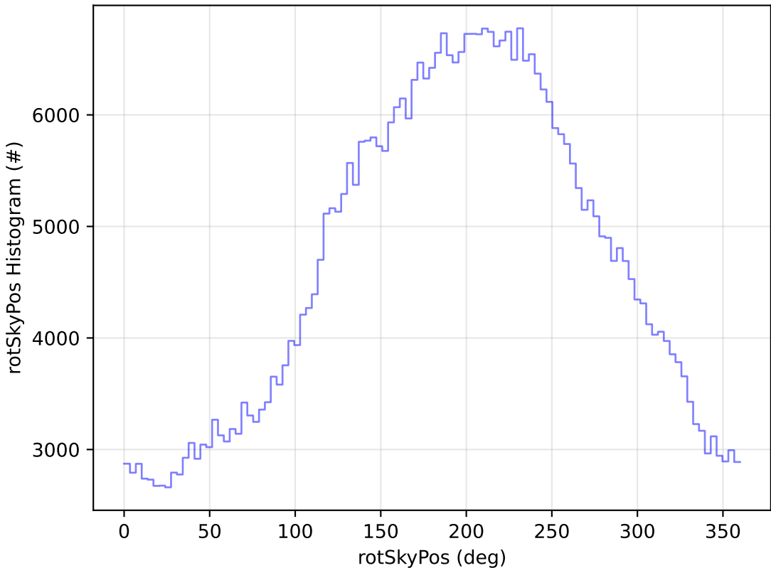
early_u_fpextra2.0_v3.4_10yrs All sky r band: rotSkyPos Histogram
