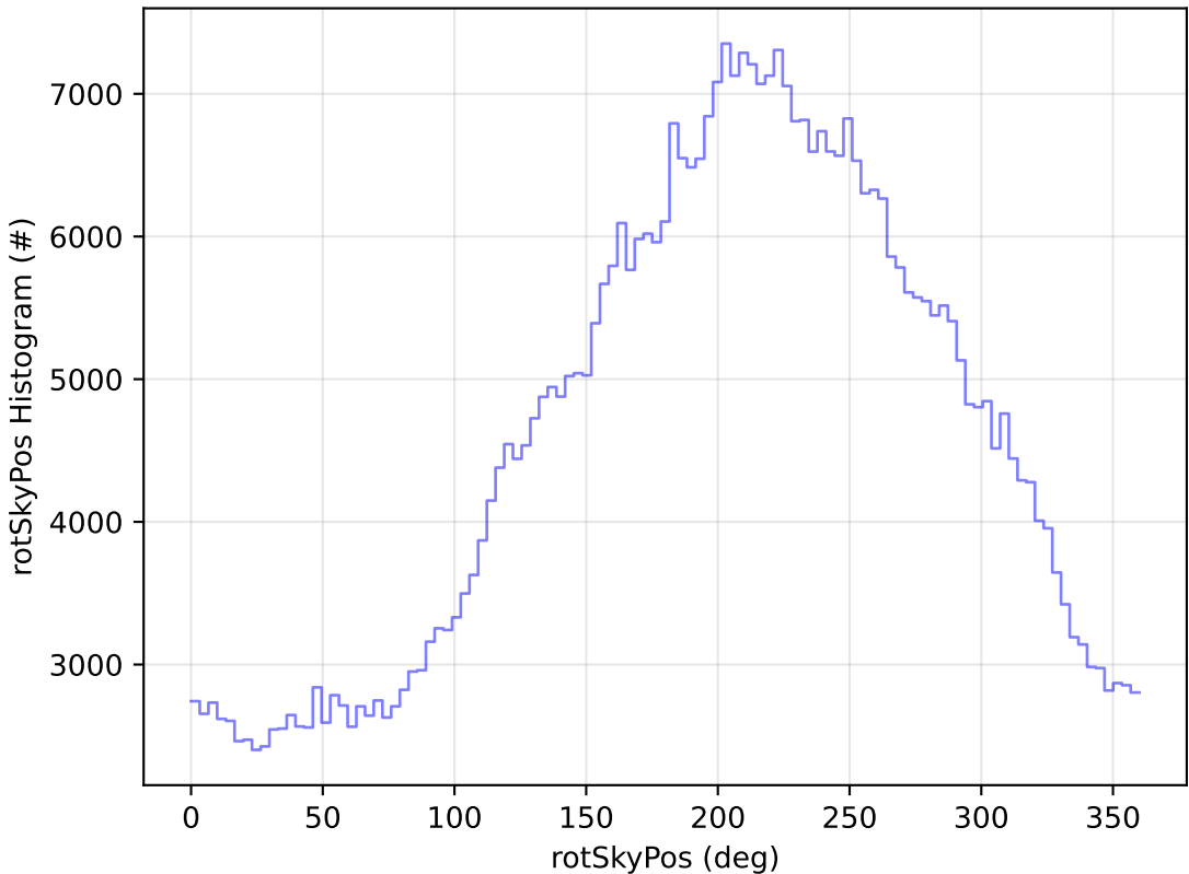
early_u_fpextra2.0_v3.4_10yrs All sky i band: rotSkyPos Histogram
