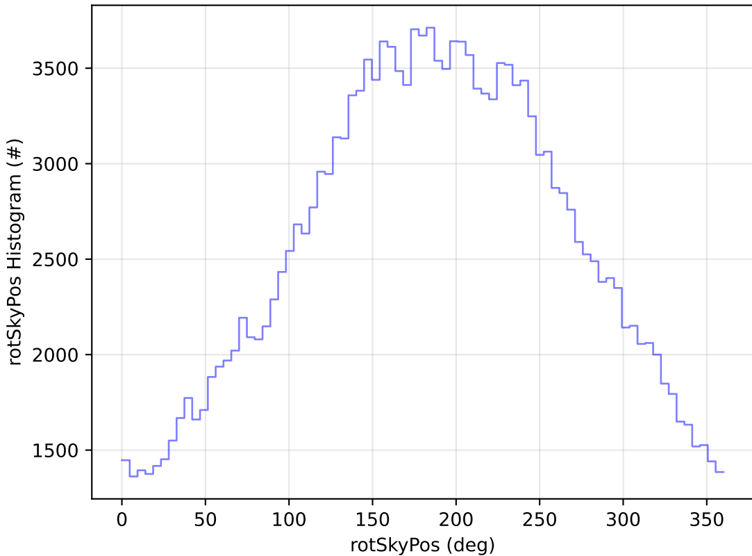
early_u_fpextra2.0_v3.4_10yrs All sky g band: rotSkyPos Histogram
