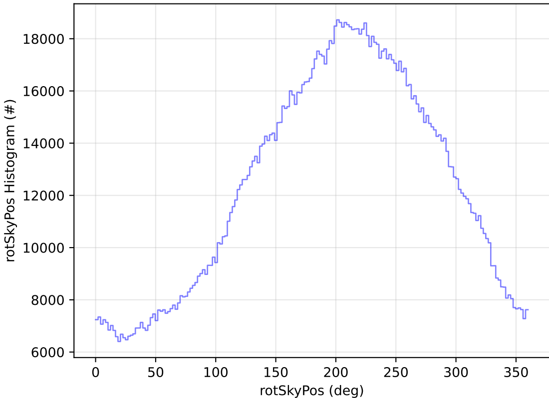
early_u_fpextra2.0_v3.4_10yrs All sky all bands: rotSkyPos Histogram
