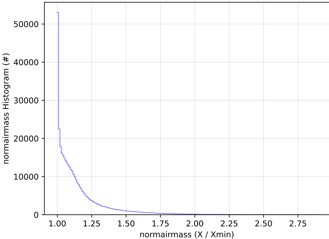
early_u_fpextra2.0_v3.4_10yrs WFD y band: normairmass Histogram
