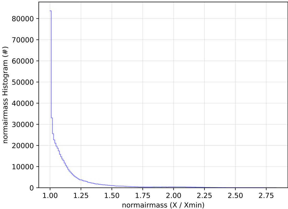
early_u_fpextra2.0_v3.4_10yrs WFD r band: normairmass Histogram
