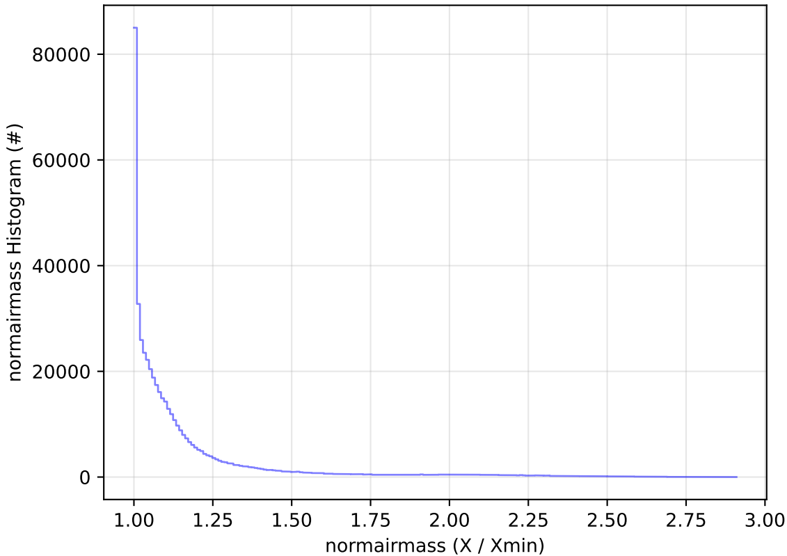
early_u_fpextra2.0_v3.4_10yrs WFD i band: normairmass Histogram
