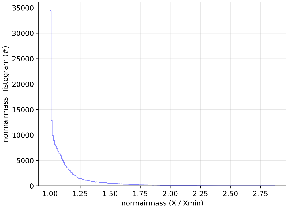
early_u_fpextra2.0_v3.4_10yrs WFD g band: normairmass Histogram
