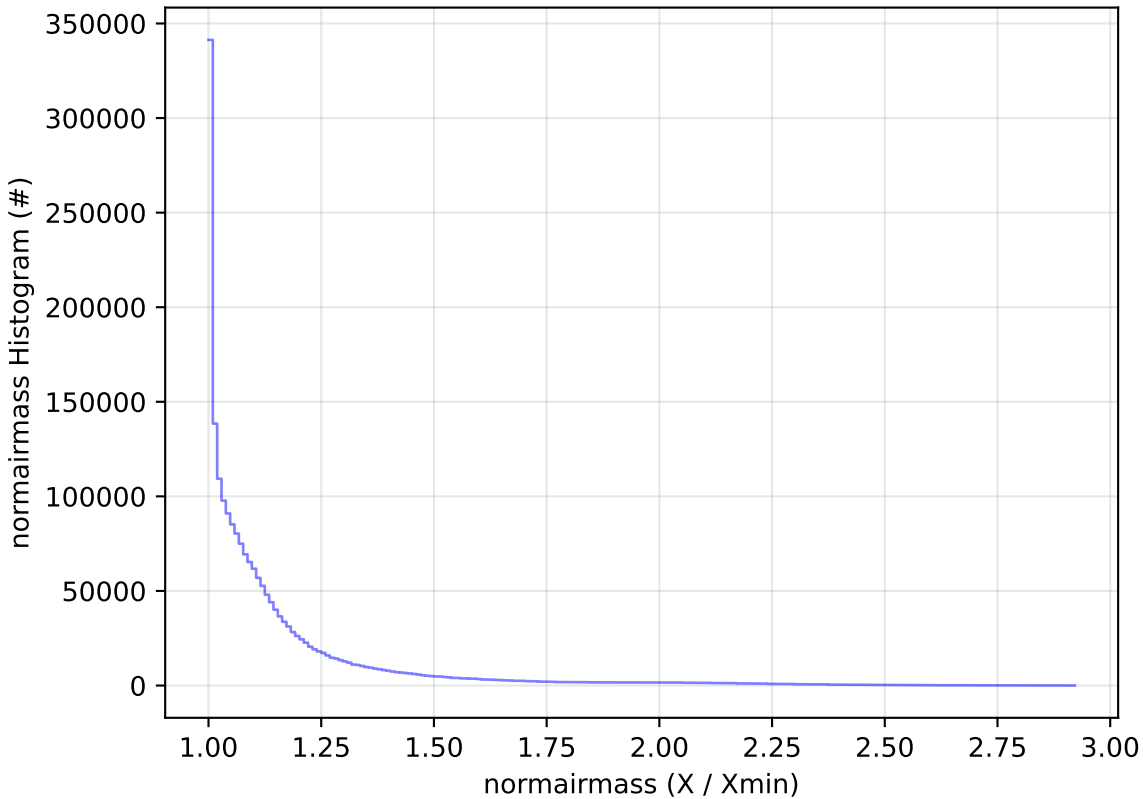
early_u_fpextra2.0_v3.4_10yrs WFD all bands: normairmass Histogram
