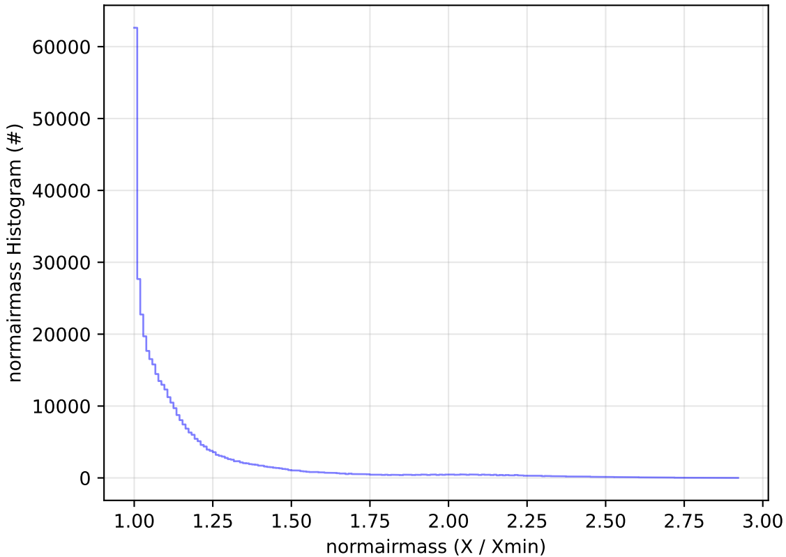
early_u_fpextra2.0_v3.4_10yrs All sky z band: normairmass Histogram
