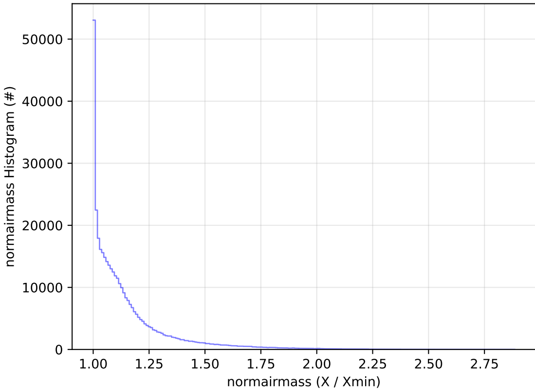
early_u_fpextra2.0_v3.4_10yrs All sky y band: normairmass Histogram
