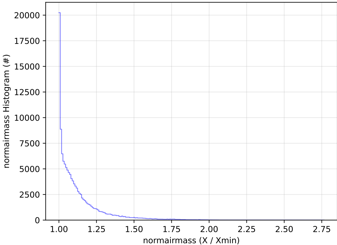
early_u_fpextra2.0_v3.4_10yrs All sky u band: normairmass Histogram
