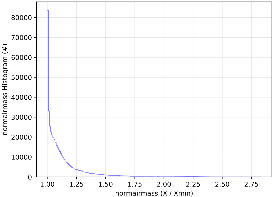
early_u_fpextra2.0_v3.4_10yrs All sky r band: normairmass Histogram
