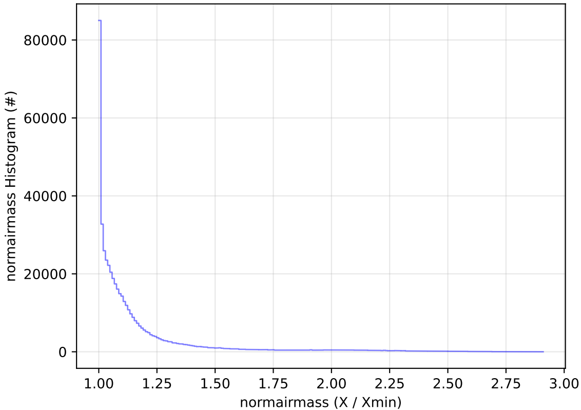
early_u_fpextra2.0_v3.4_10yrs All sky i band: normairmass Histogram
