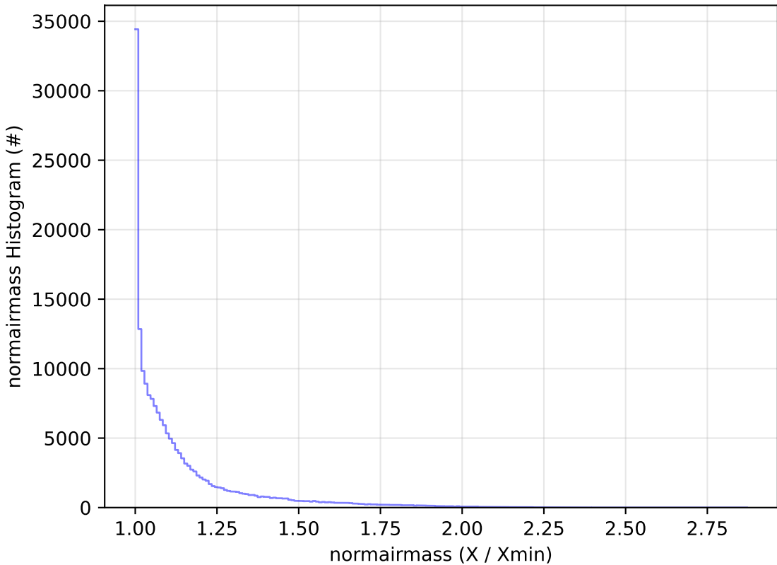
early_u_fpextra2.0_v3.4_10yrs All sky g band: normairmass Histogram
