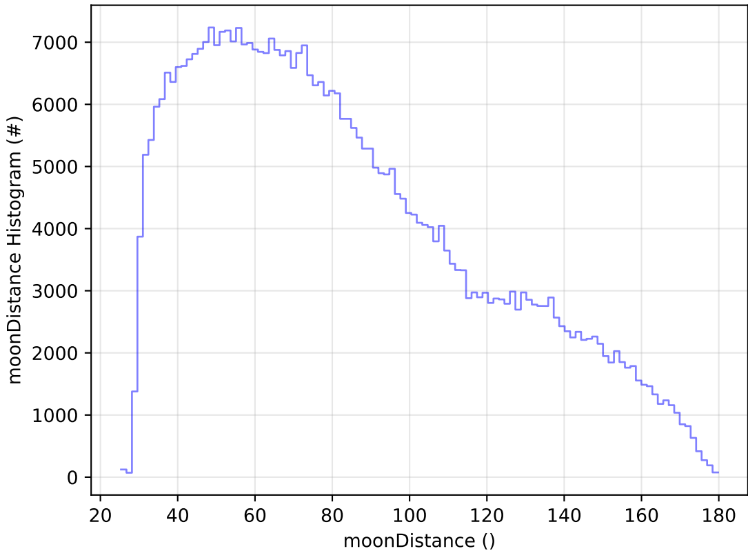
early_u_fpextra2.0_v3.4_10yrs WFD z band: moonDistance Histogram
