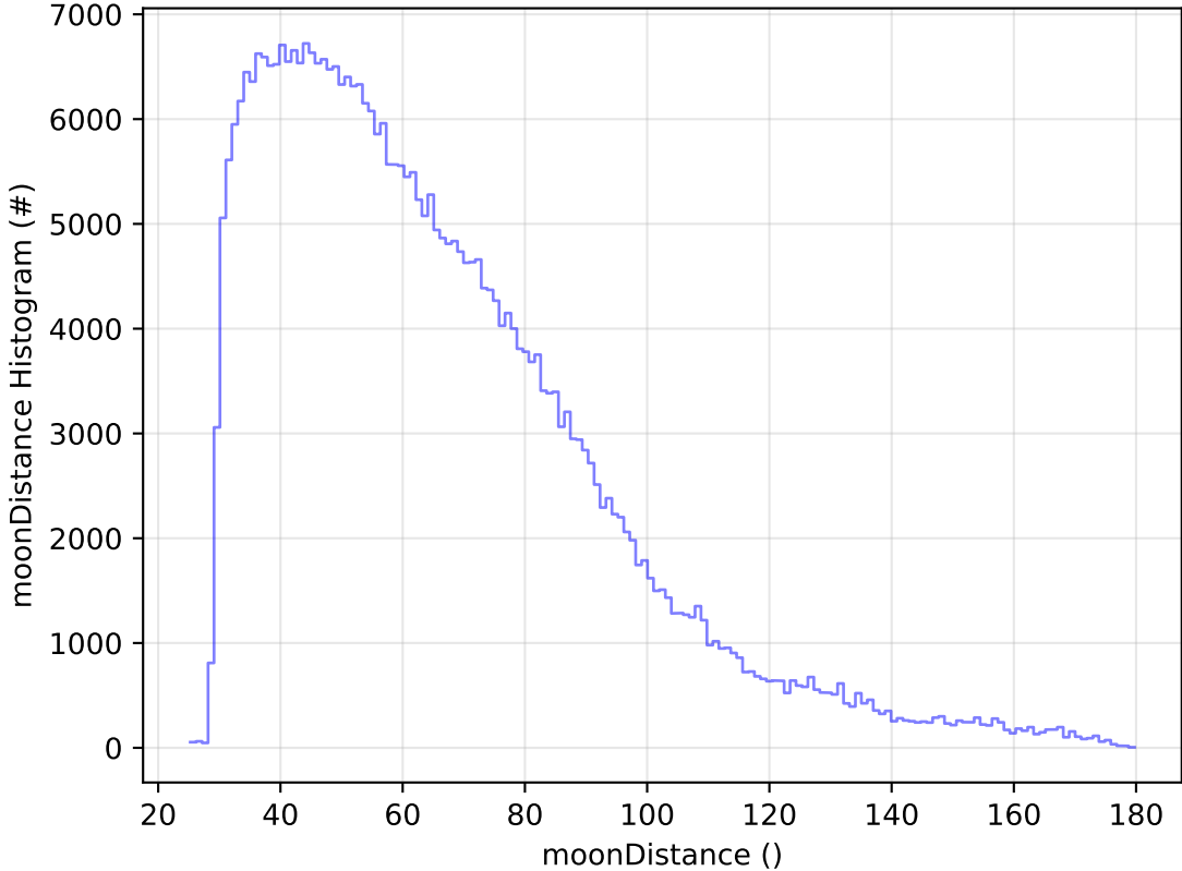
early_u_fpextra2.0_v3.4_10yrs WFD y band: moonDistance Histogram
