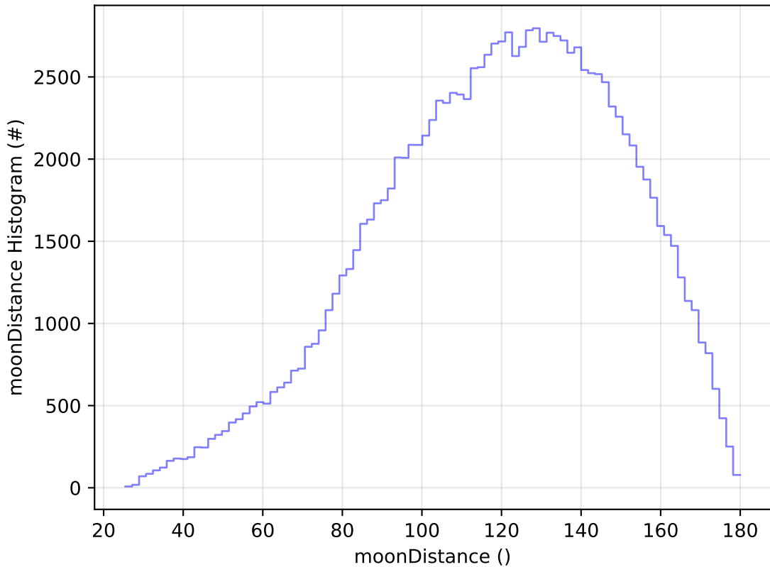
early_u_fpextra2.0_v3.4_10yrs WFD u band: moonDistance Histogram
