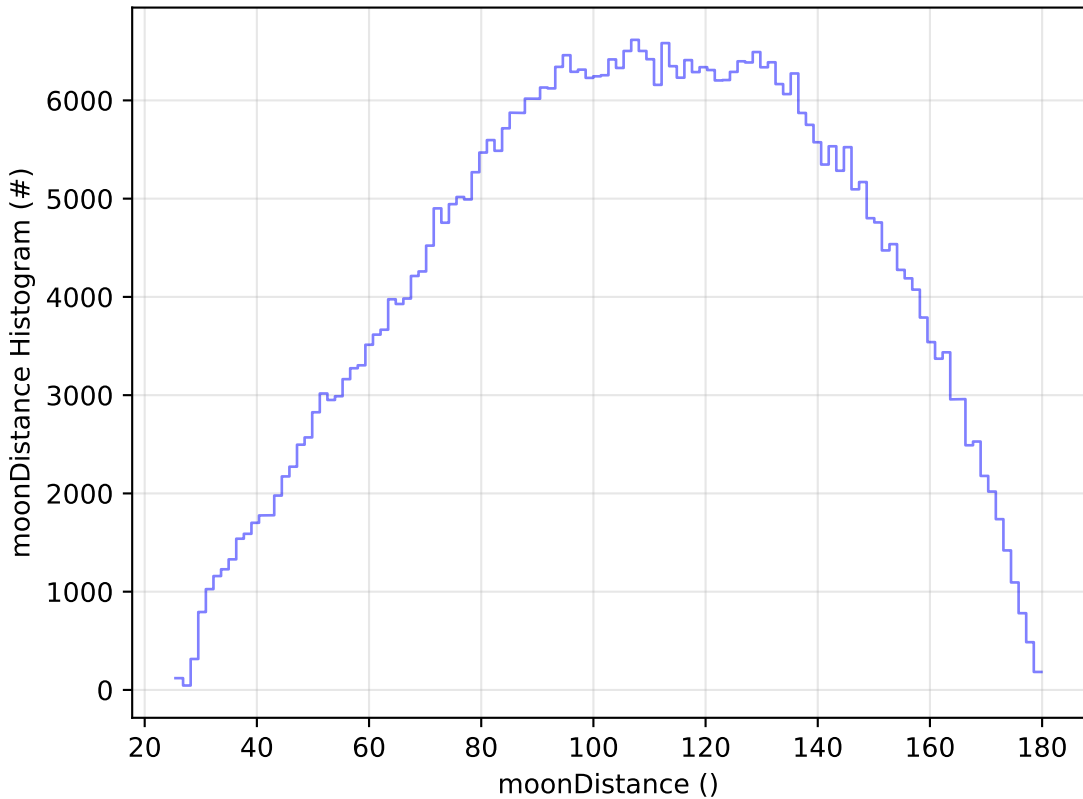
early_u_fpextra2.0_v3.4_10yrs WFD r band: moonDistance Histogram
