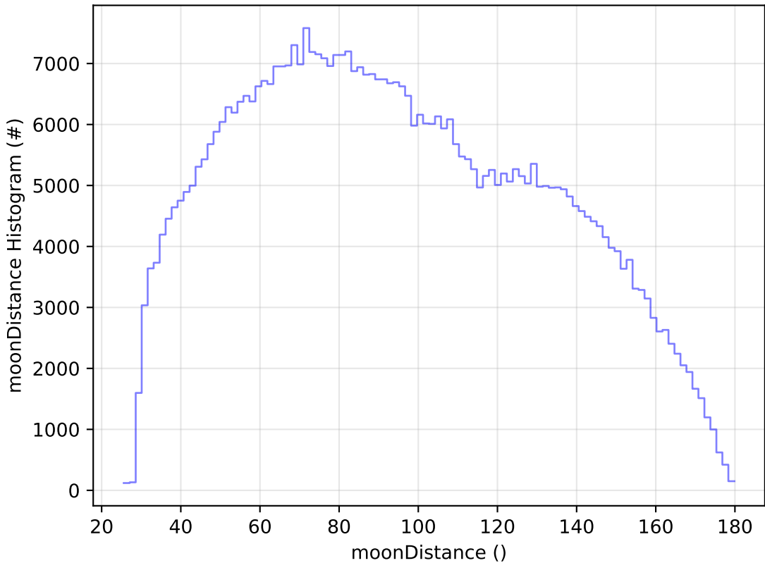
early_u_fpextra2.0_v3.4_10yrs WFD i band: moonDistance Histogram
