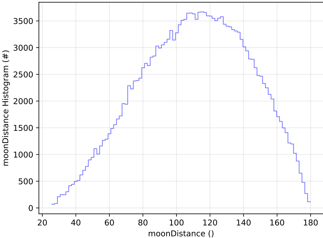
early_u_fpextra2.0_v3.4_10yrs WFD g band: moonDistance Histogram
