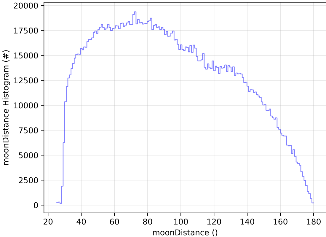
early_u_fpextra2.0_v3.4_10yrs WFD all bands: moonDistance Histogram
