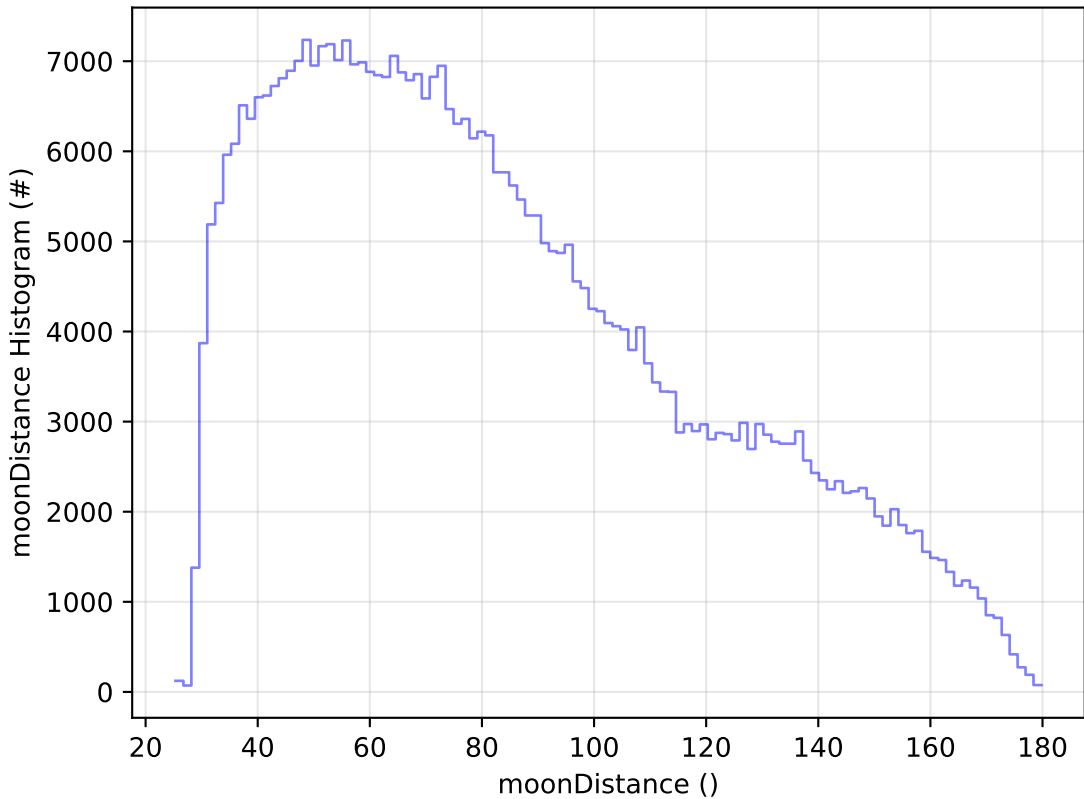
early_u_fpextra2.0_v3.4_10yrs All sky z band: moonDistance Histogram
