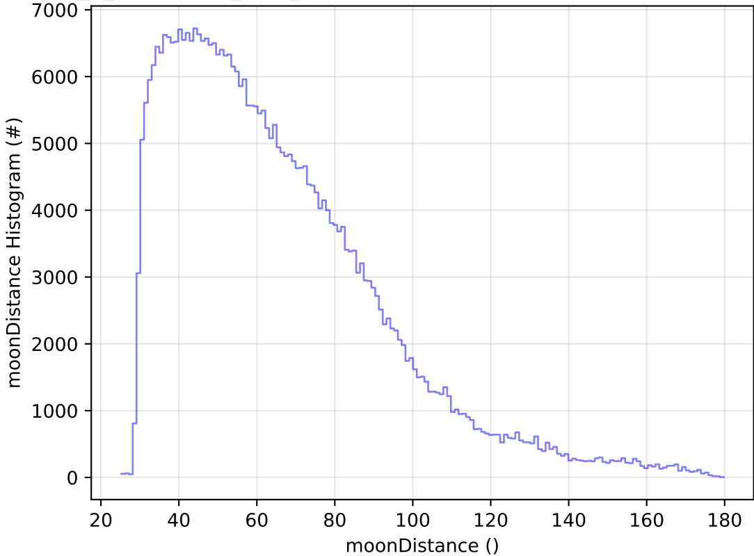
early_u_fpextra2.0_v3.4_10yrs All sky y band: moonDistance Histogram
