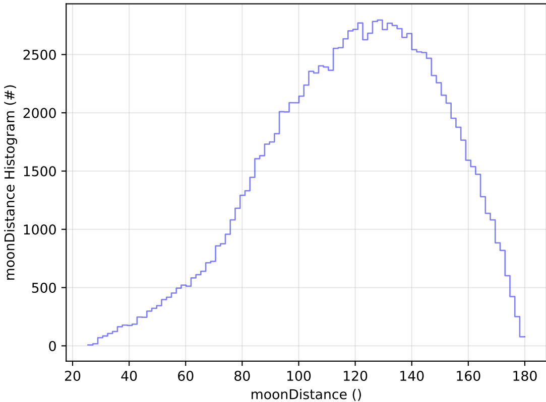
early_u_fpextra2.0_v3.4_10yrs All sky u band: moonDistance Histogram
